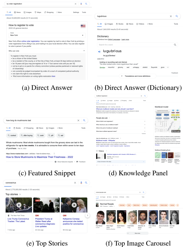
Figure 1: Examples of extracted results components.
